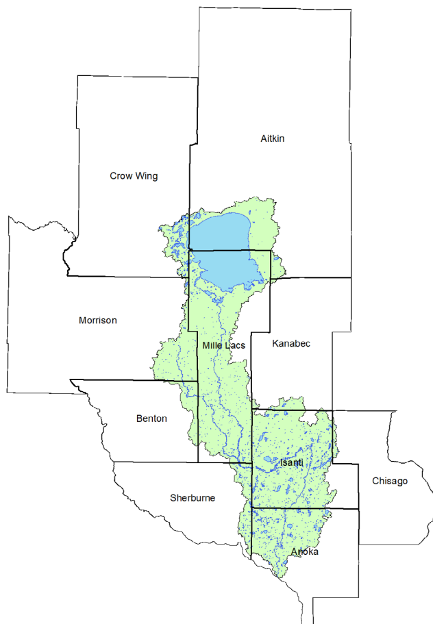
Figure 1: Watershed Map
